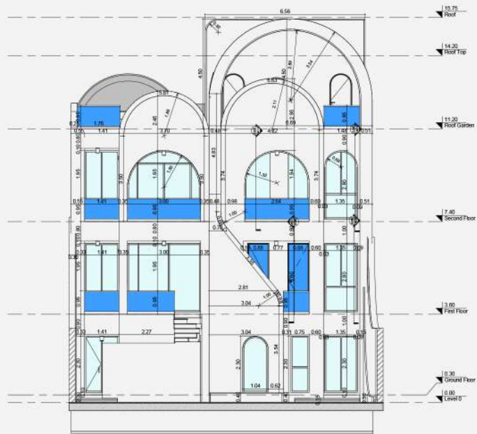
North Elevation
