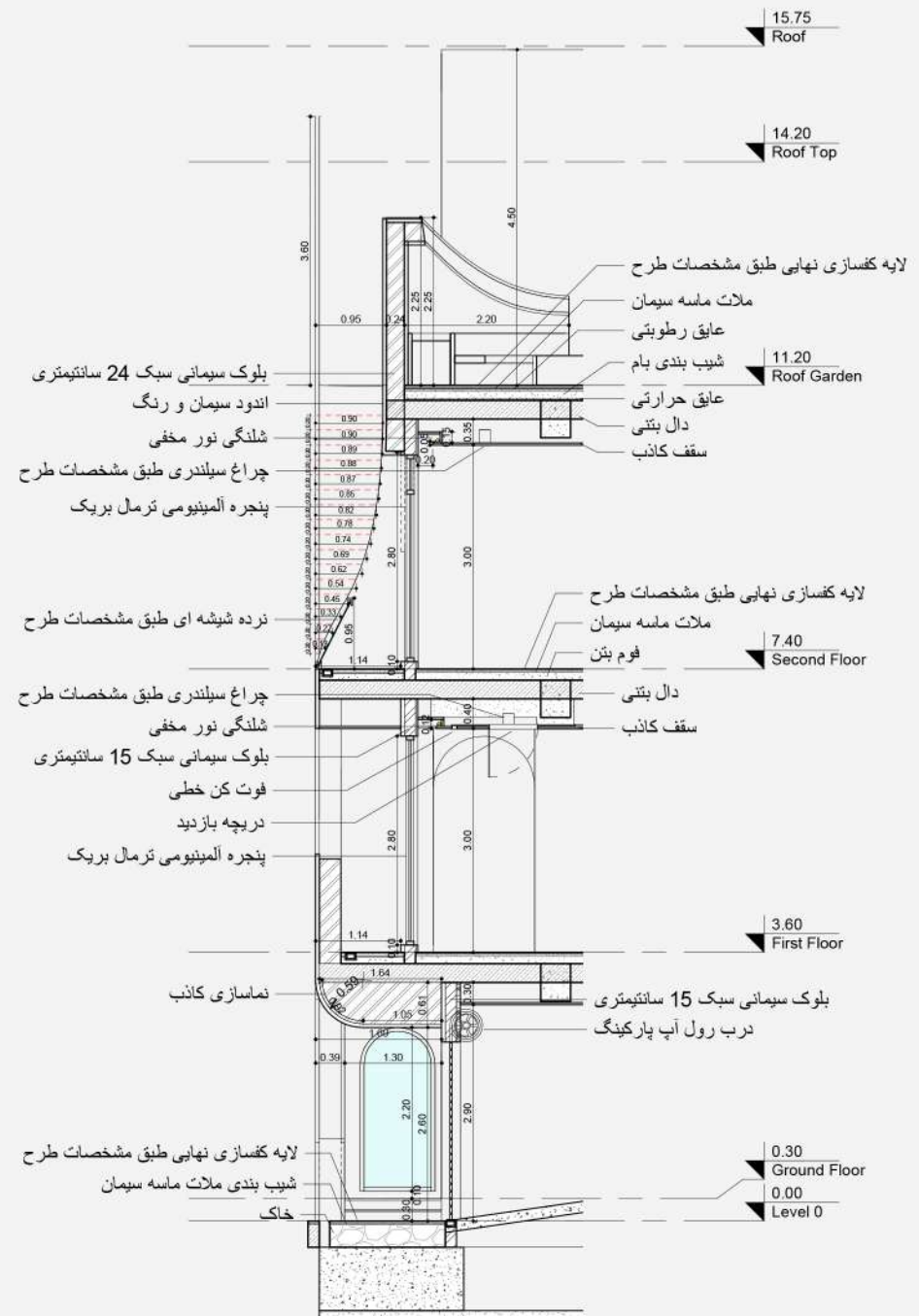
Wal Section
