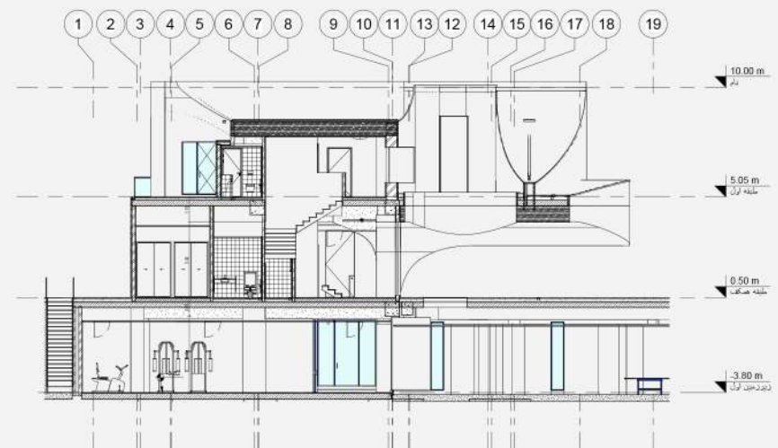
Sec B-B
