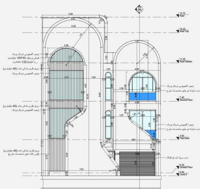
South Elevation
