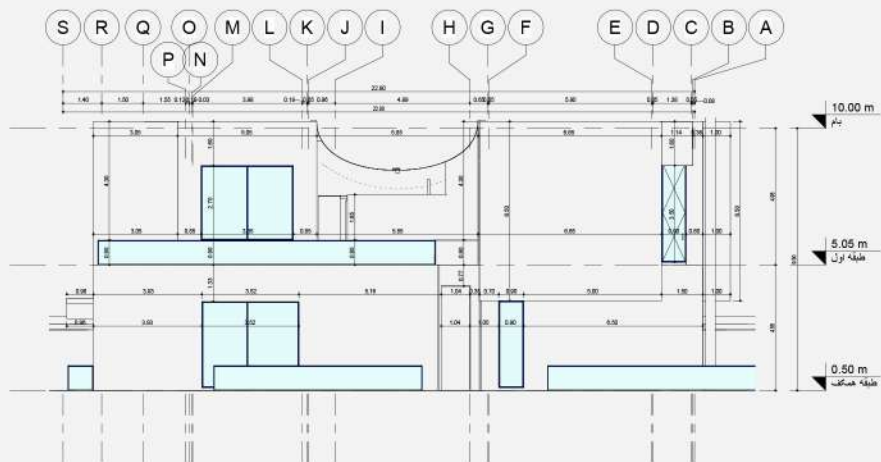
North Elevation
